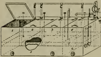
FIG. 3. TANK FOR SATURATING WOOL WASTE.
